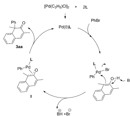
Scheme 1. Proposed catalytic cycle for palladium-catalyzed arylative dearomatization of naphthols.
